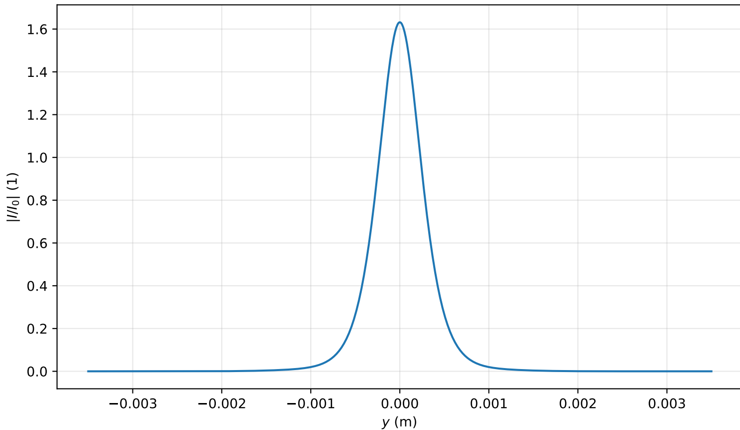
Intensity profile I(x=0, y, z=2.309)/I_0 , P_{in}=0.9P_{cr} , artificial time
